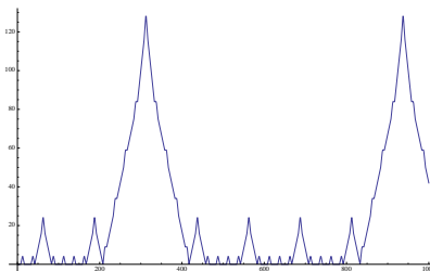
FIGURE 1. The 5-adic valuation of A_n
